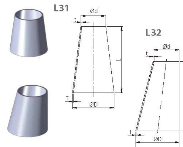
WELD REDUCERS
