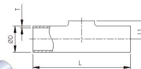
7WO LONG EQUAL PULL WITHOUT STRAIGHT WELD TEE
