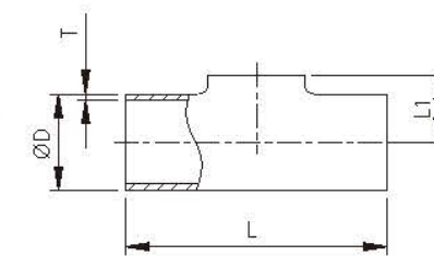
7WWO SHORT EQUAL PULL WITHOUT STRAIGHT WELD TEE
